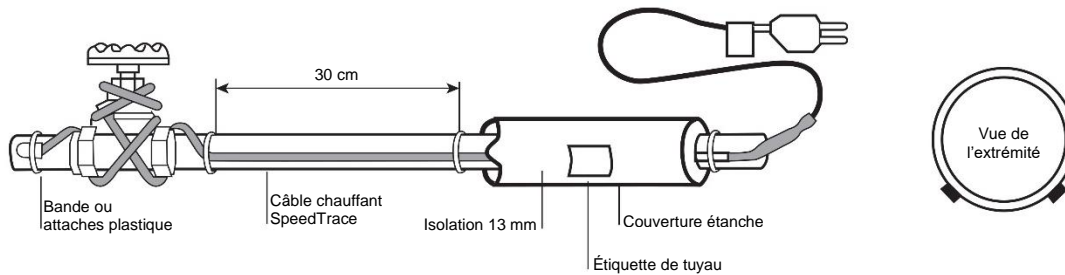
Figure 2 Installation en spirale
