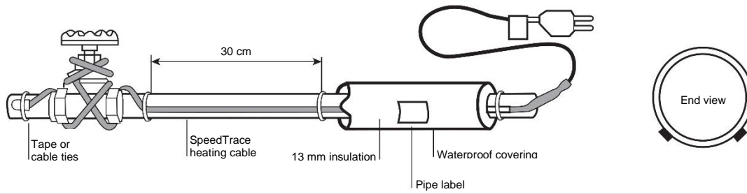
Figure 2 Spiral-traced installation
